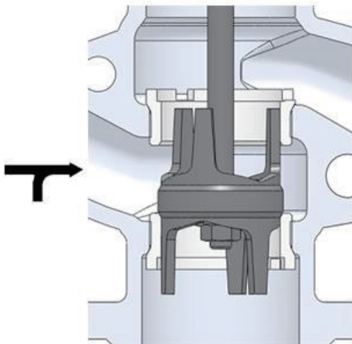
⑥ Three-way mixing design, two passages mix fluid onto one passage.
