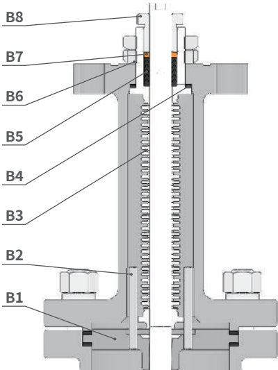
Metal Bellow Seal
