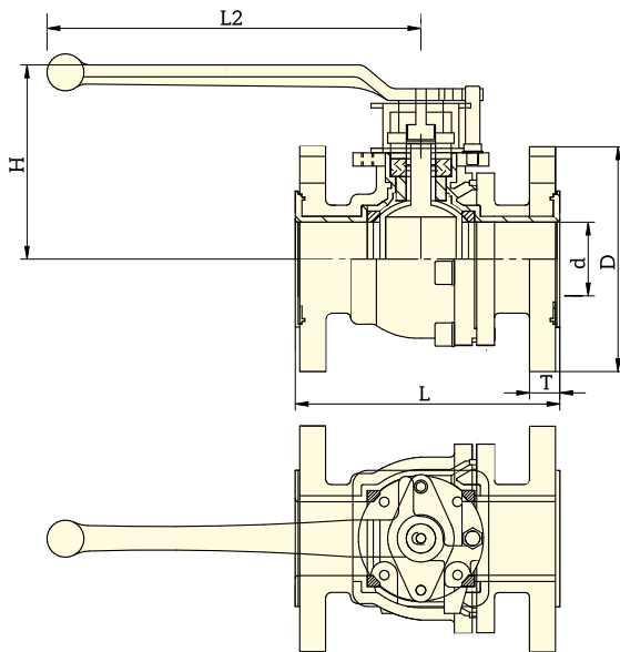
SECTIONAL VIEW
